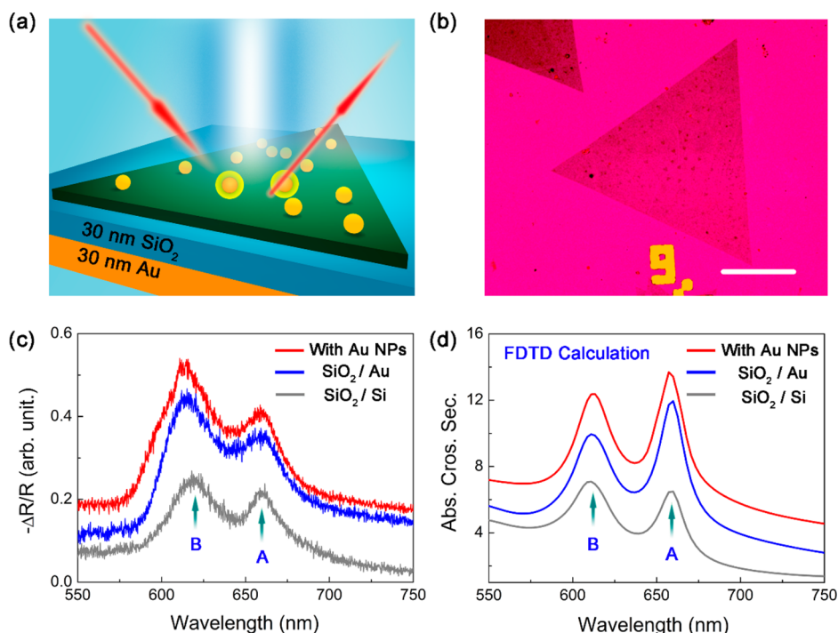
Figure 1. (a) Schematic of \text{MoS}_2 -Au hybrid film under 532 nm laser excitation and white light illumination. The substrate consists of 30 nm \text{SiO}_2 film on a 30 nm thick Au mirror. (b) Optical image of the \text{MoS}_2 monolayer under a 100\times objective lens (scale bar is 30 \mu\text{m} ). (c) Absorption spectra of the \text{MoS}_2 -Au hybrid film on a \text{SiO}_2/\text{Si} substrate (red) and \text{MoS}_2 film on \text{SiO}_2/\text{Au} (blue) and on \text{SiO}_2/\text{Si} (gray). The concentration of the Au NPs is 10 \text{ mg L}^{-1} . (d) Absorption cross section simulated by FDTD.
