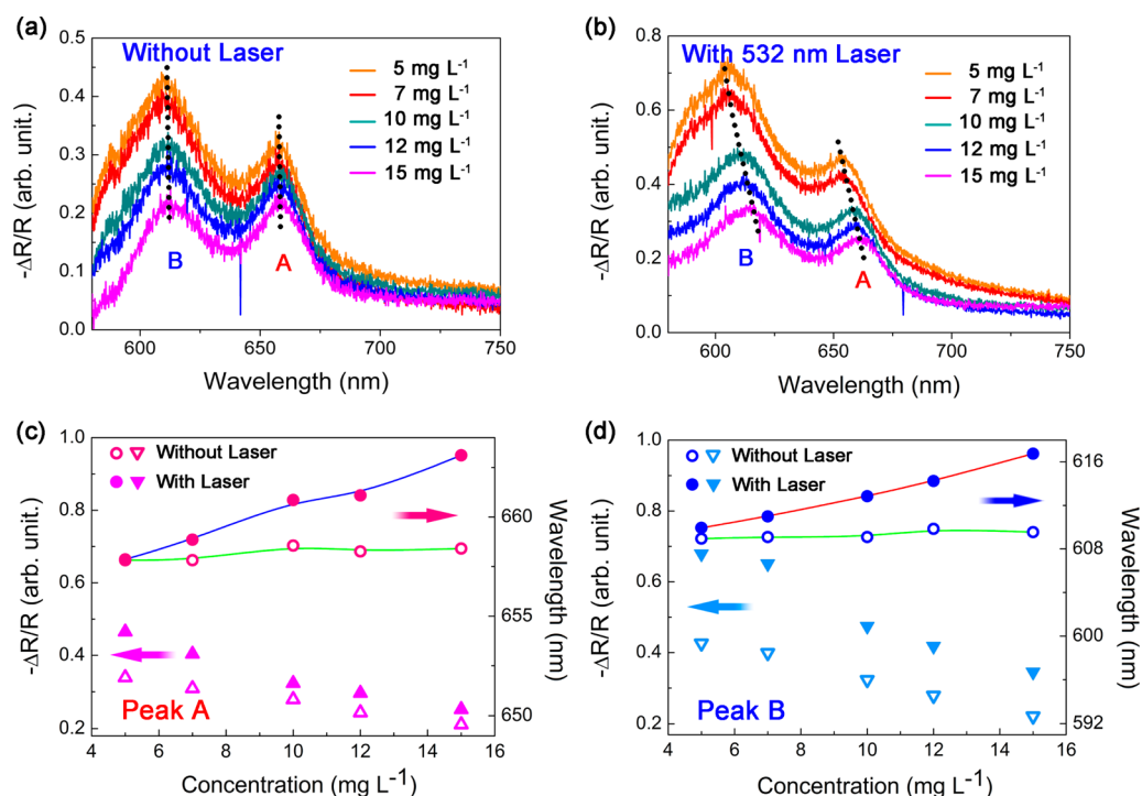
Figure 2. Absorption spectra without (a) and with (b) 532 nm laser illumination as a function of Au NP concentrations ranging from 5 to 15 mg L -1 . Peak wavelength (circles) and intensity variations (triangles) of peak A (c) and peak B (d) with (solid symbols) and without (hollow symbols) laser excitation. The laser power is 1 mW.
