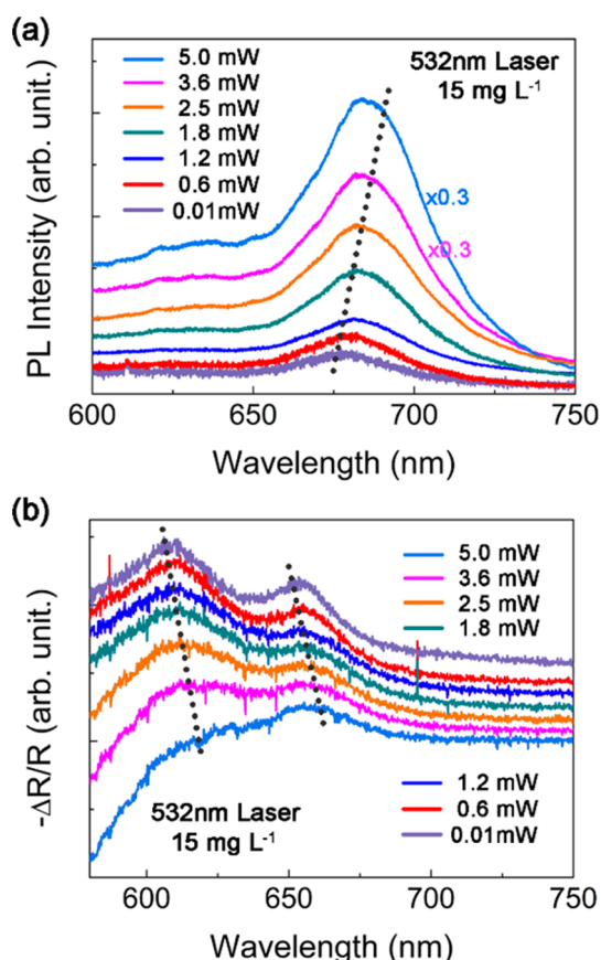
Figure 3. (a) PL spectra and (b) absorption spectra of the MoS 2 structure with 15 mg L -1 NP concentration for laser powers ranging from 0.01 to 5 mW. The excitation laser wavelength is 532 nm.
