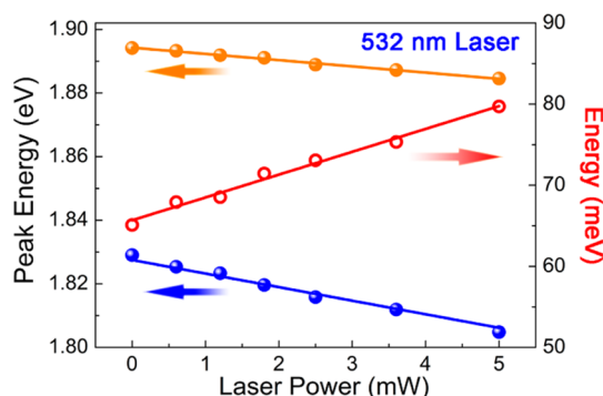
Figure 6. Absorption peak A (orange) and luminescence peak (blue) from Figure 3 as a function of laser power. The red line is the energy difference between the absorption and PL peak energy for each of the incident laser powers that changed from 0.01 to 5 mW.
