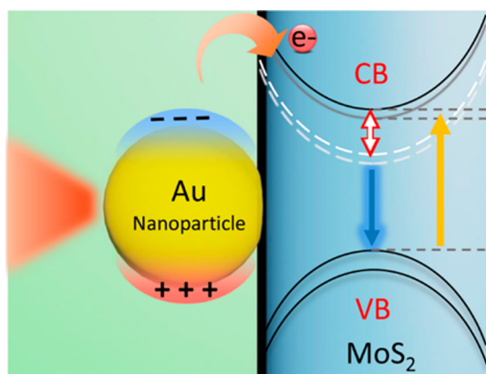
Figure 5. Schematic view of the interaction between Au nanoparticles and MoS 2 monolayers. The white dashed line represents excitonic energy level. The yellow arrow represents the absorption process of the peak A, an electronic transition from the upper spin–orbit split valence band to the conduction band (peak B is due to excitation from the lower spin–orbit split valence band but not shown). The blue arrow represents the PL emission. The hollow arrow represents the tunable binding energy change of the exciton that is controlled by the doping level of the conduction band.
